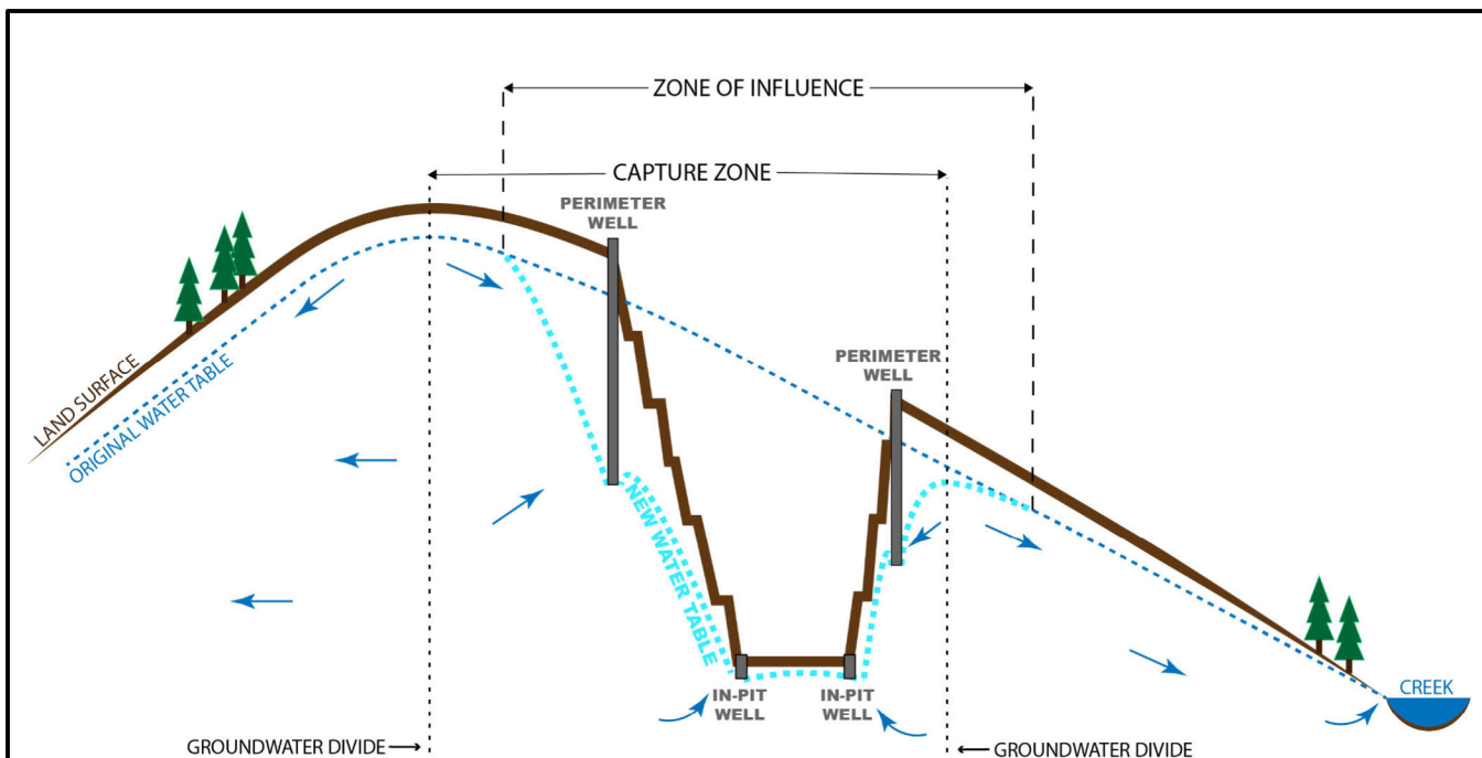
PIT DEWATERING SCHEMATIC: OPERATIONS (NOT TO SCALE)
