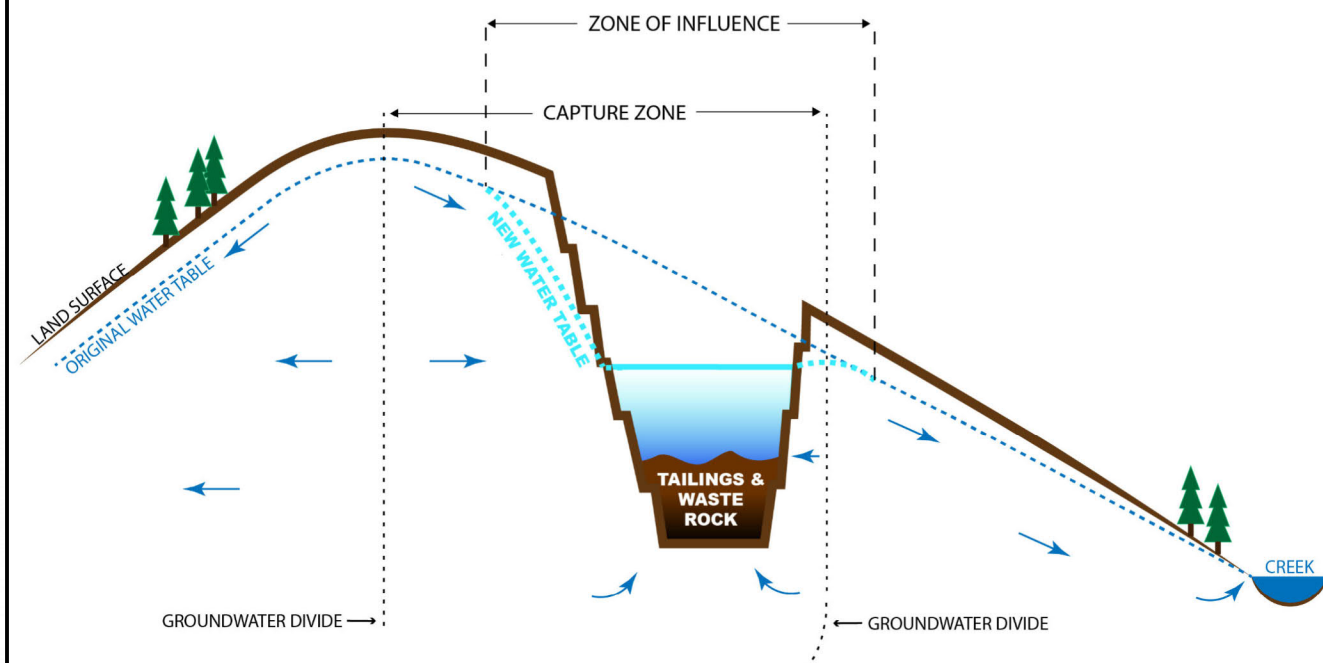
PIT LAKE SCHEMATIC: POST CLOSURE (NOT TO SCALE)
