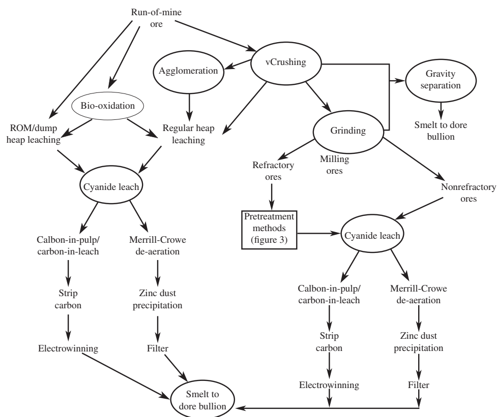
Figure 8. Processing technologies for gold ore. Source: U.S. Bureau of Mines, 1994, fig. 2.
