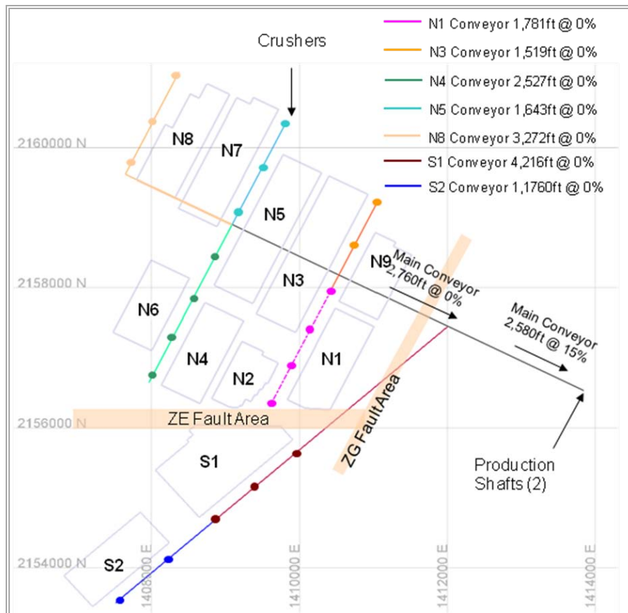
Figure 18.1.17 Conveyor Schematic
