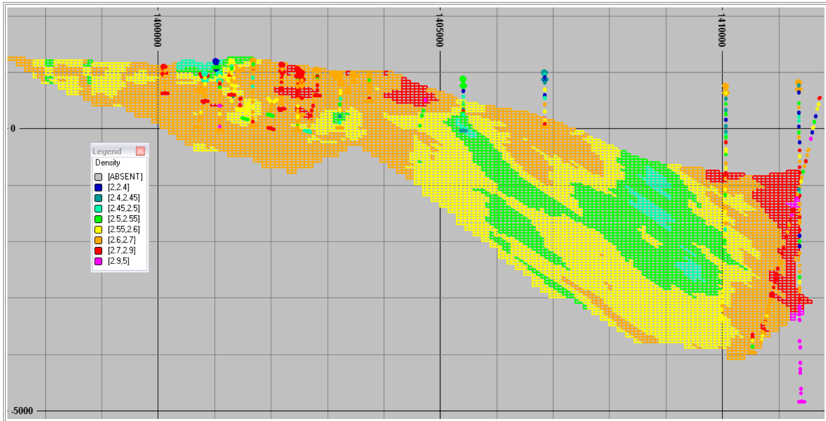
Figure 17.11.12 Ordinary Kriging Density (SG) Section at 2158000 ft N with Corresponding Sample Data at \pm 150 ft Clipping Distance
