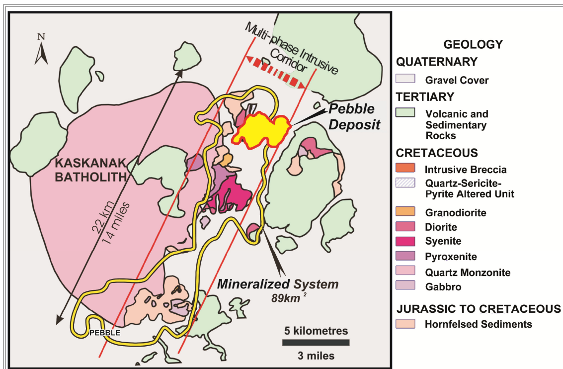
Figure 7.1.2 District Geology of the Pebble Deposit Showing the Major Lithological Units and Relative Ages
