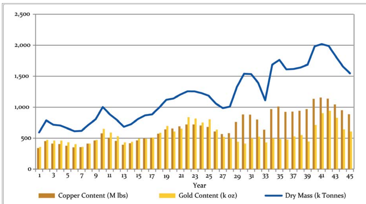
Figure 18.8.1 Copper-Gold Concentrate Produced – 45-Year Reference Case
